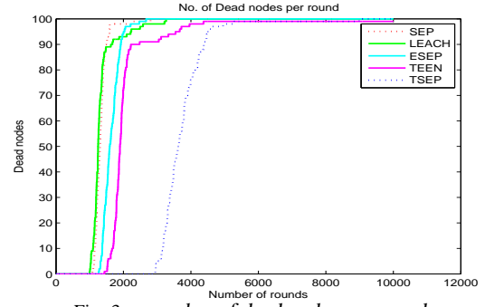
Fig. 3. number of dead nodes per round.
